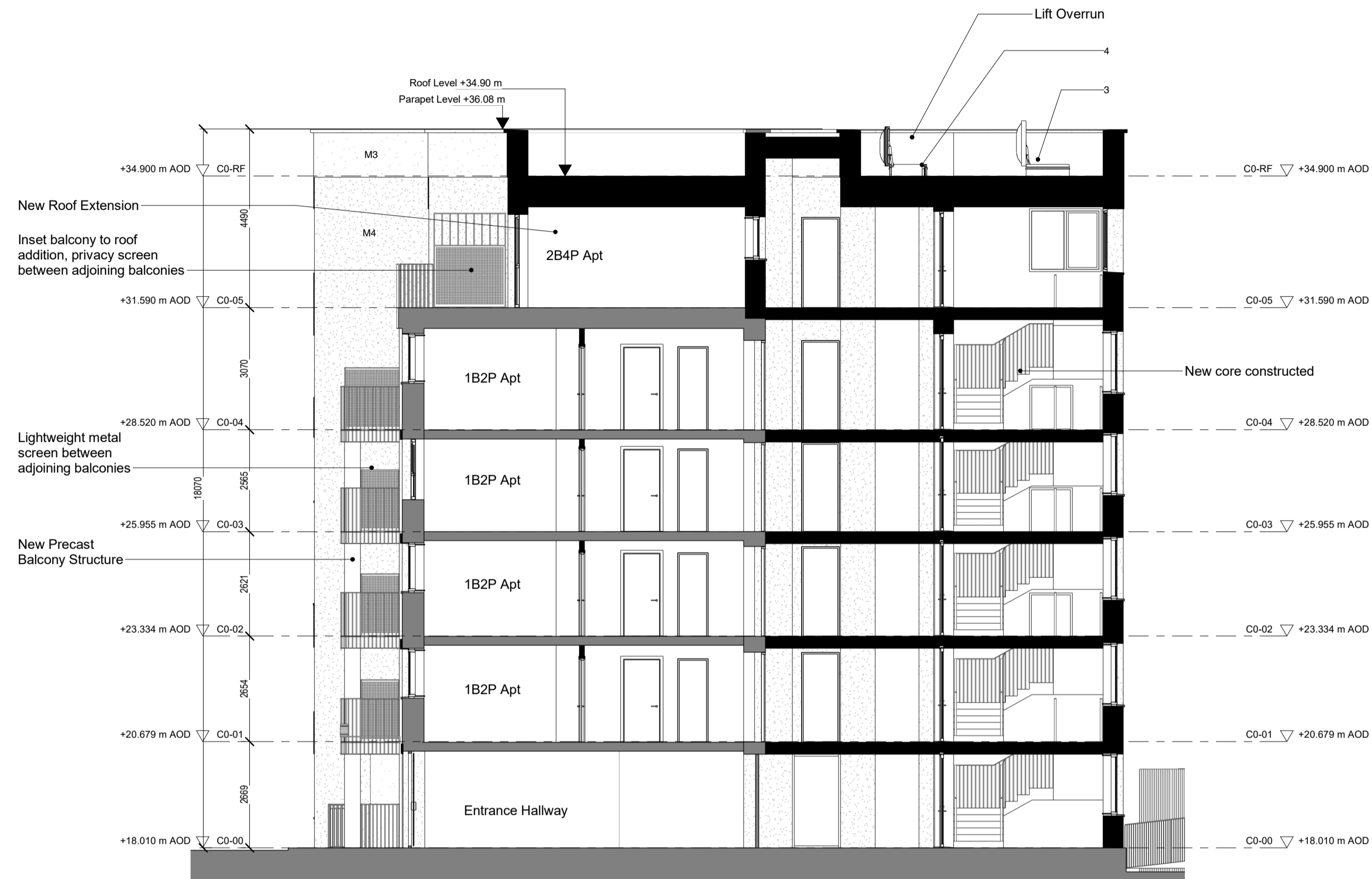
Section E-E, C0 Stair Section
