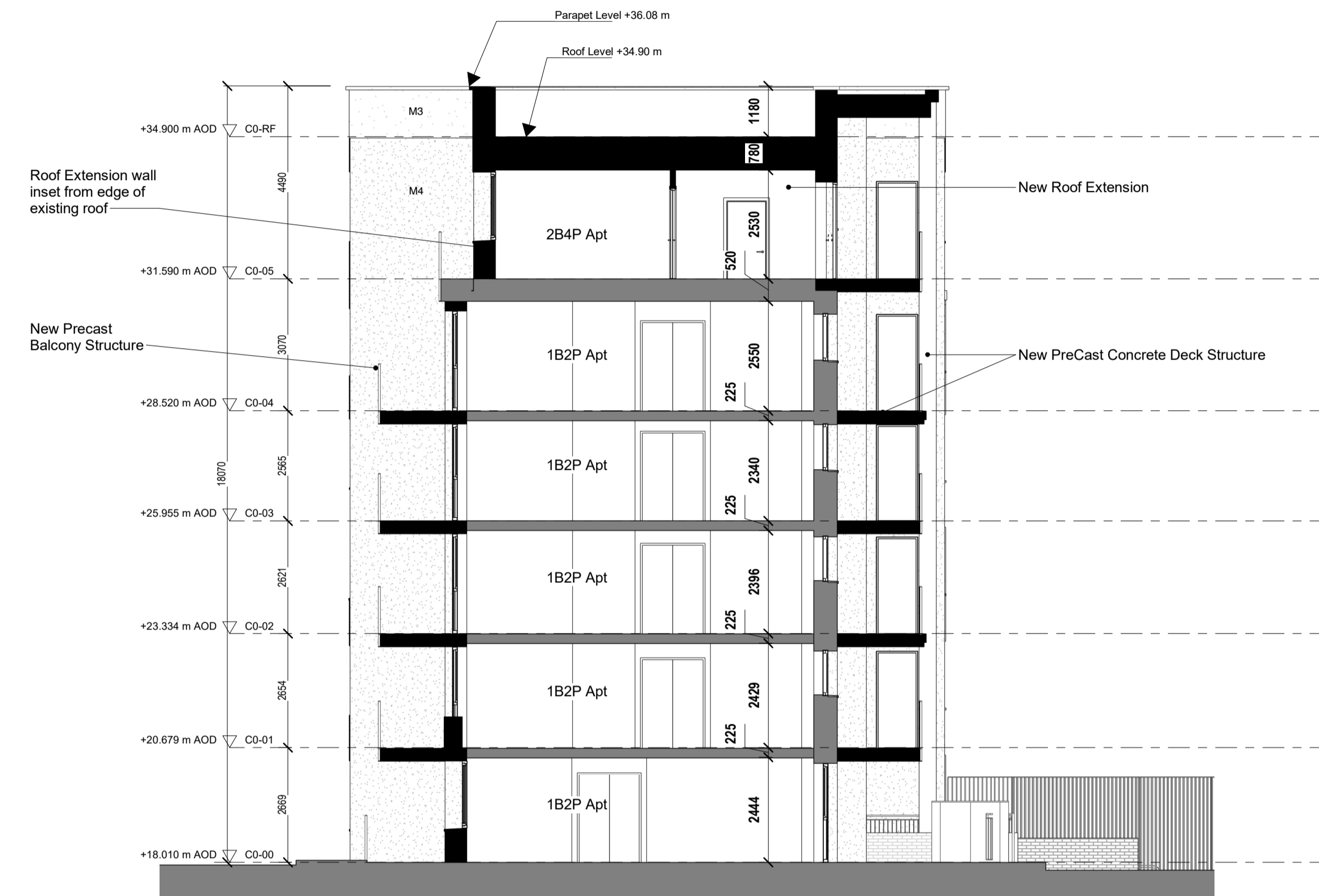
Section F-F, C0 Typical Section
