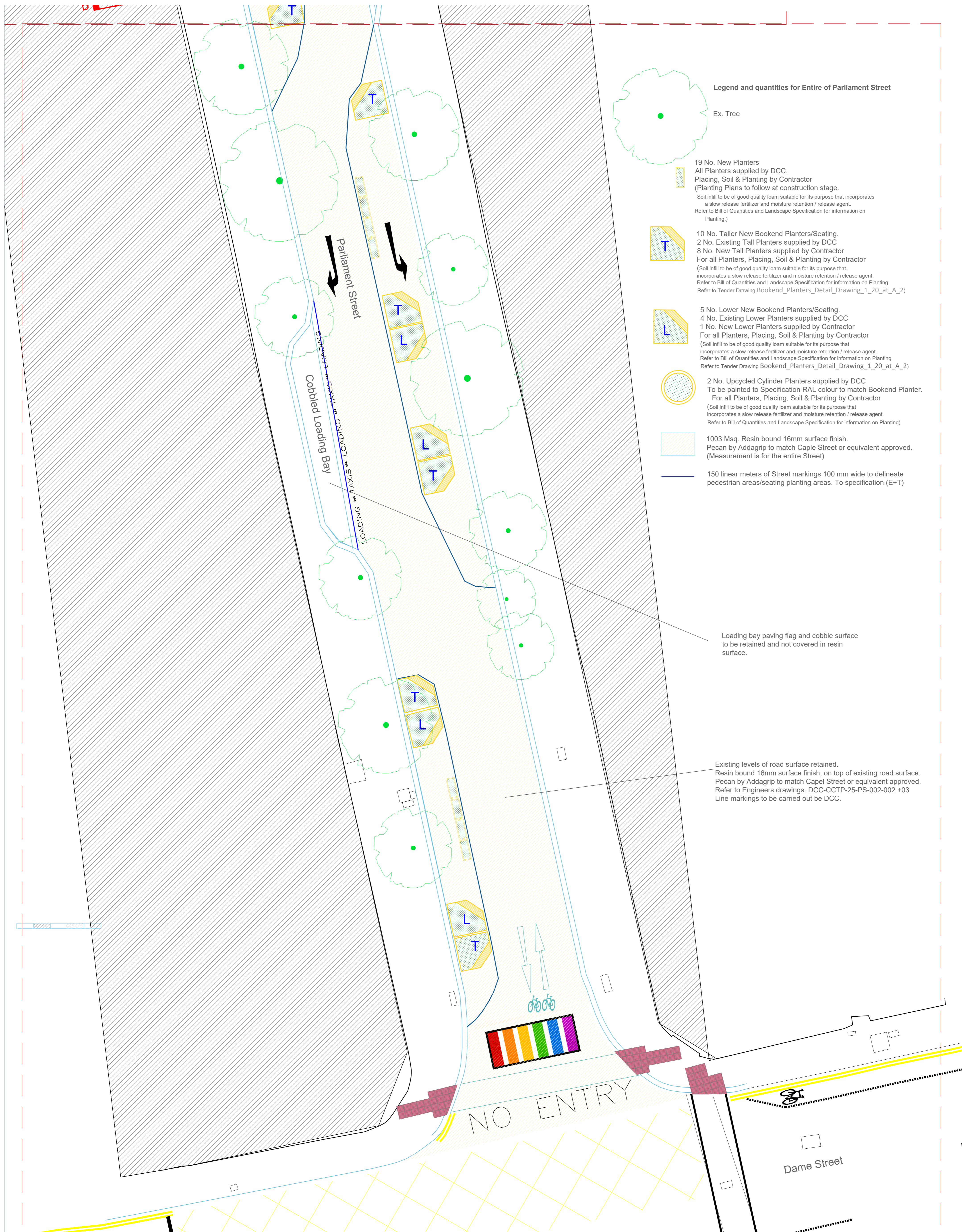
PLAN VIEW OF PARLIAMENT STREET SOUTH SCALE: 1:100 @A1
