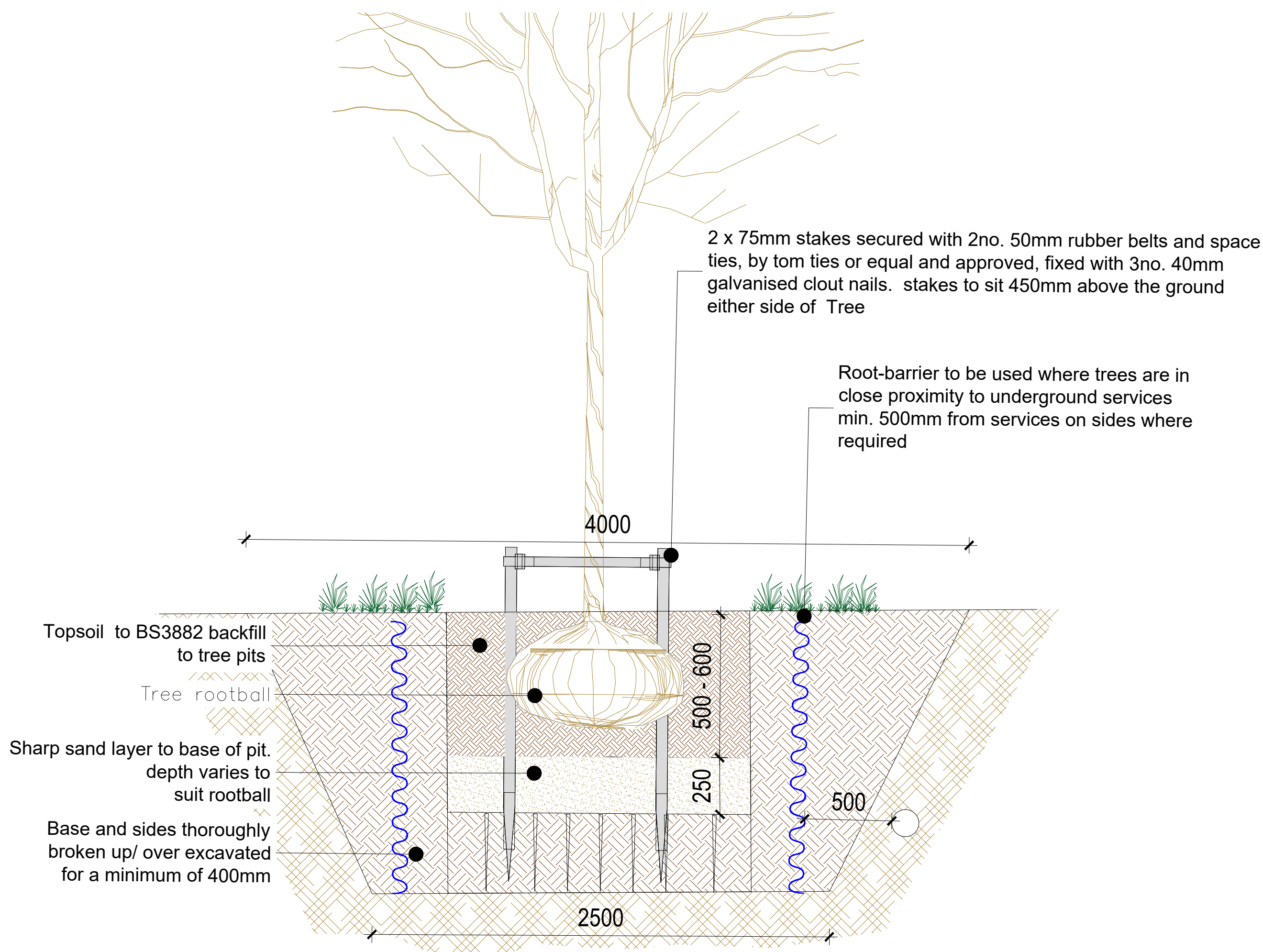
Typical Tree Planting Detail
