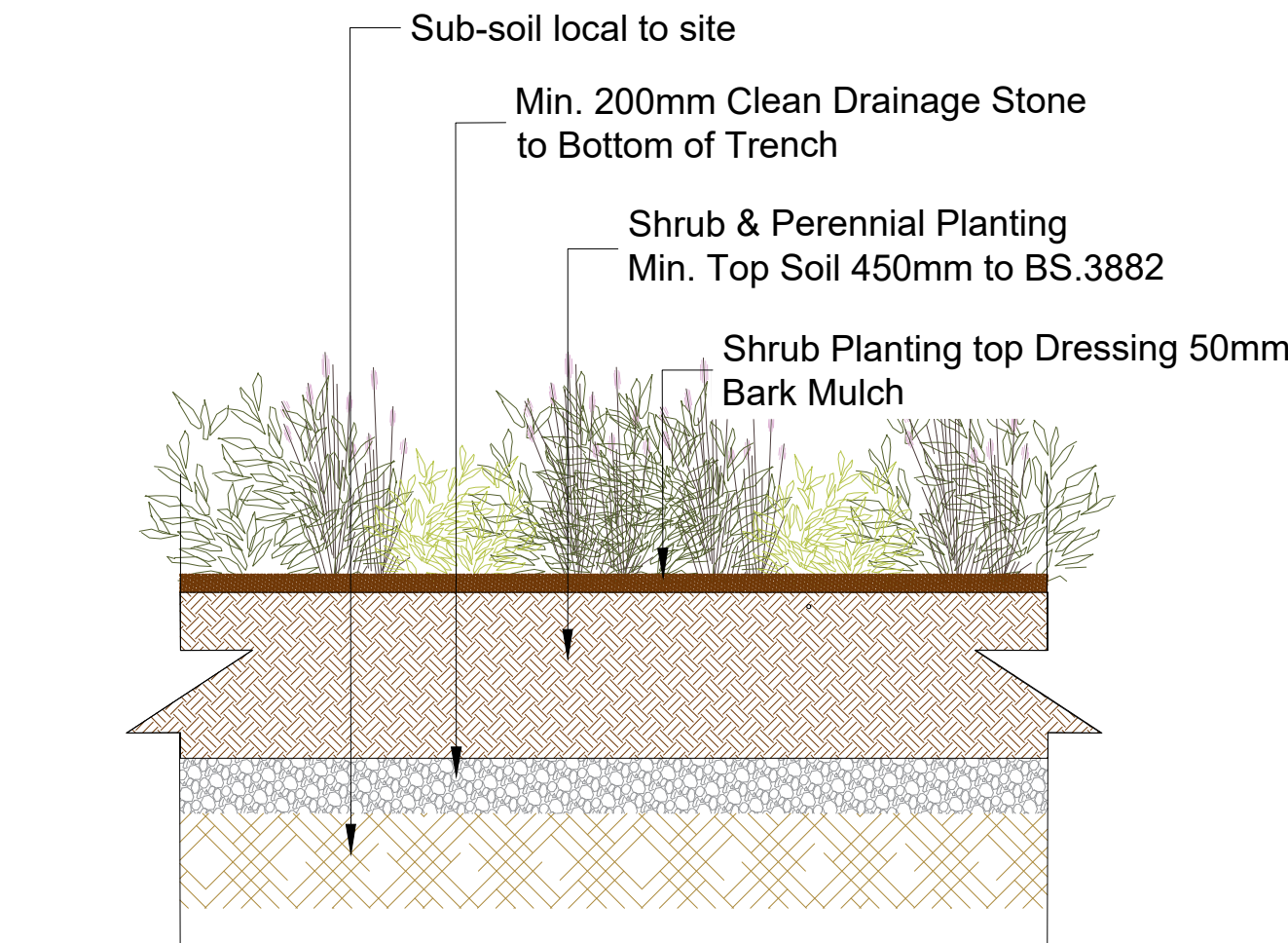
Typical Shrub Planting Detail
