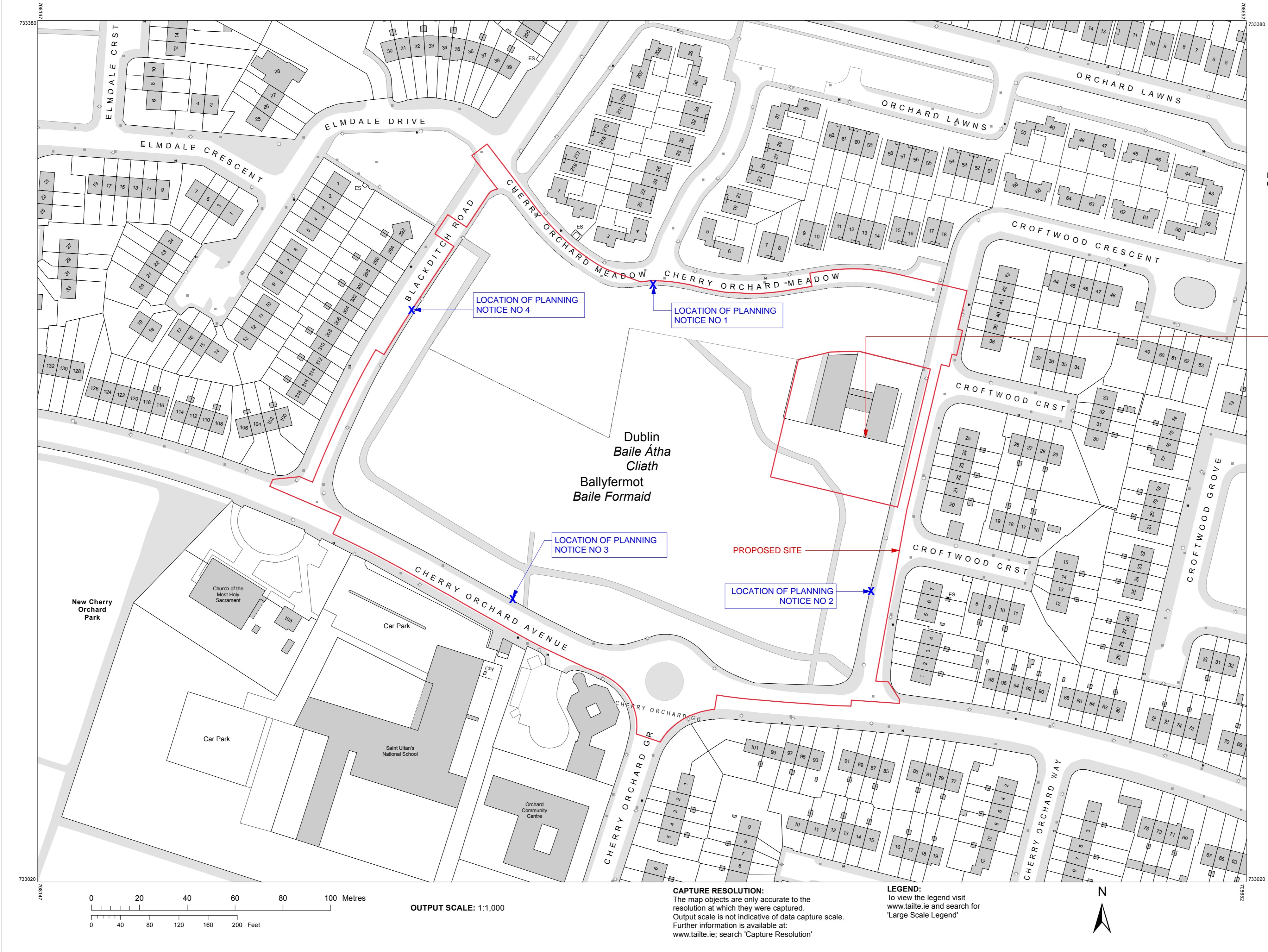
Proposed Site Location Plan Scale: 1:1000
