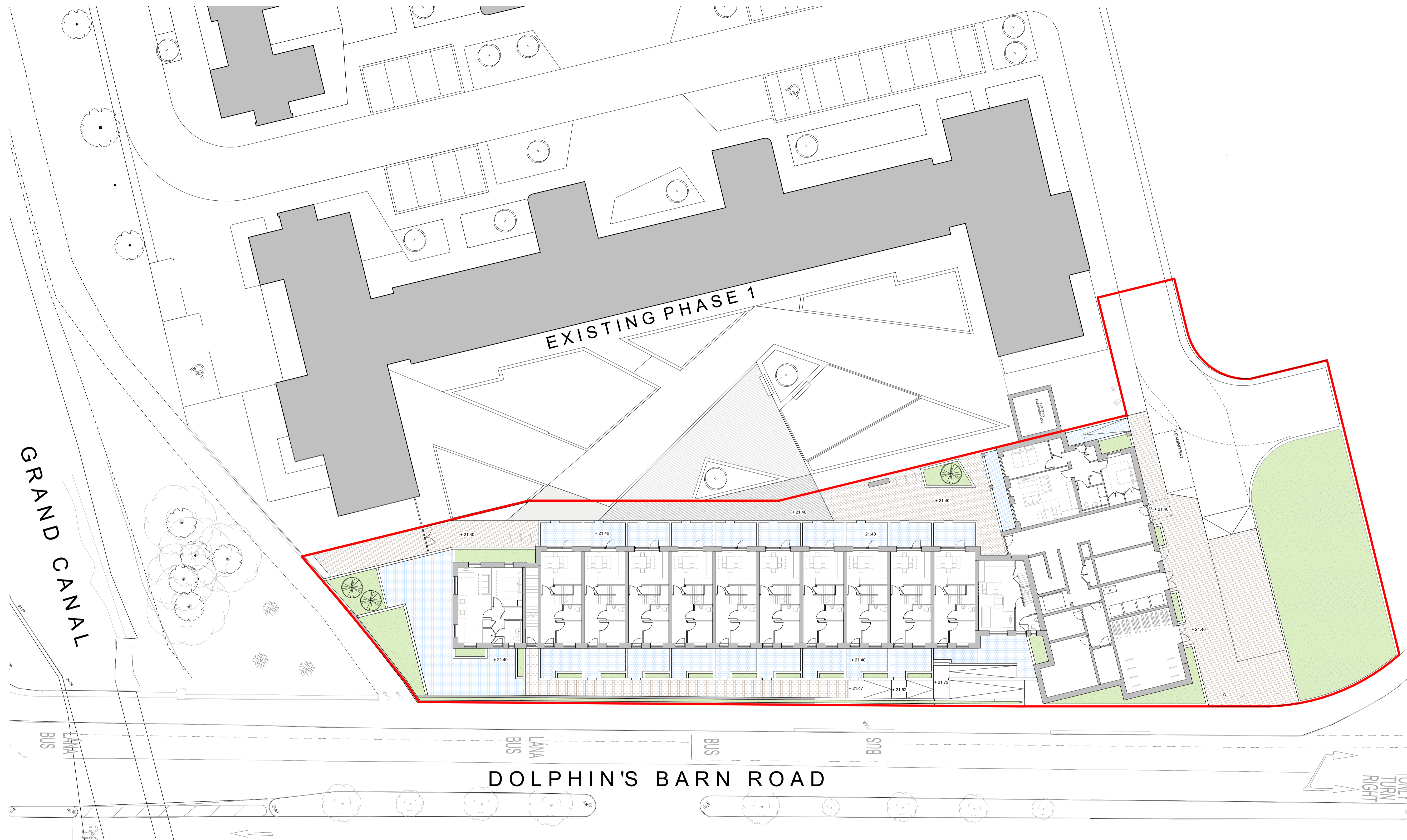
1 Proposed Landscape Plan 1:200
